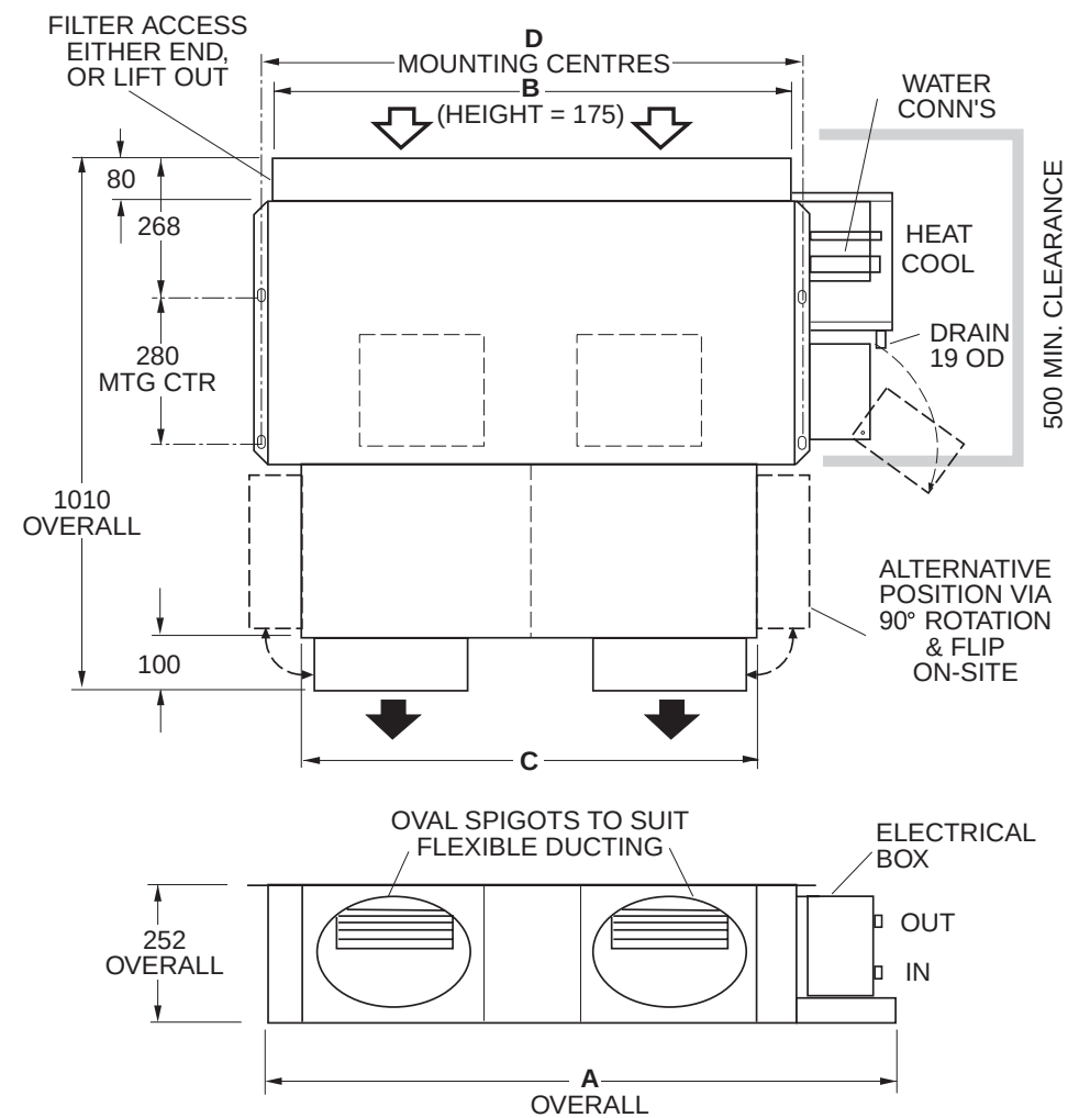
Model IXDL 90Y Shown.
